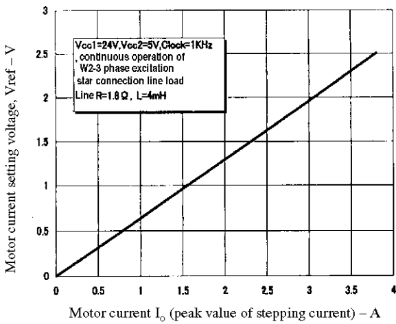
Figure 4. V_{ref} - I_o
