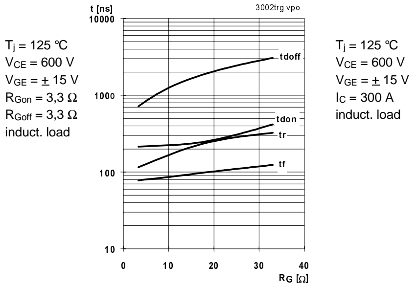
Fig. 16 Typ. switching times vs. gate resistor R_G
