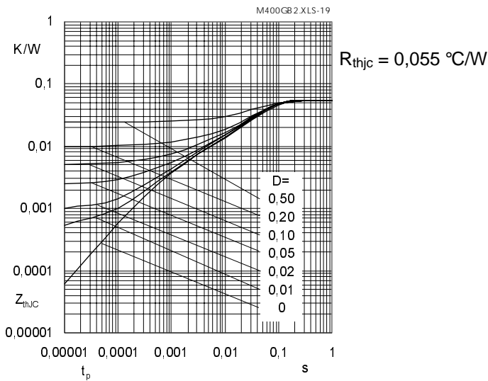
Fig. 19 Transient thermal impedance of IGBT Z_{thJC} = f(t_p) ; D = t_p / t_c = t_p \cdot f
