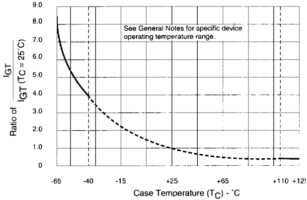
Figure 6 — Normalized DC Gate-Trigger Current vs Case Temperature
