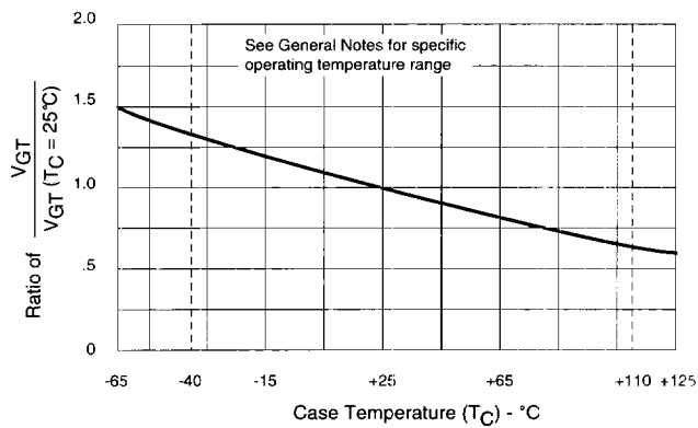
Figure 8 — Normalized DC Gate-Trigger Voltage vs Case Temperature
