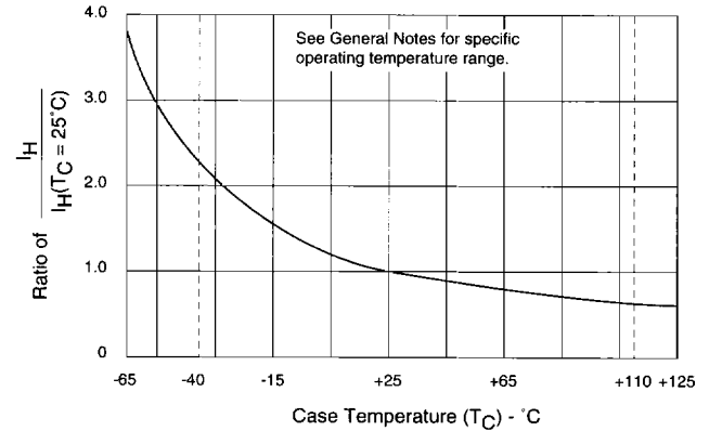
Figure 9 — Normalized DC Holding Current vs Case Temperature
