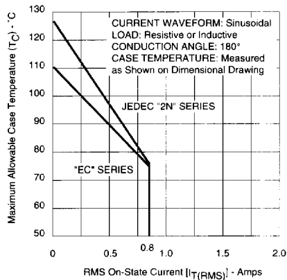
Figure 1A — Maximum Allowable Case Temperature vs RMS On-State Current
