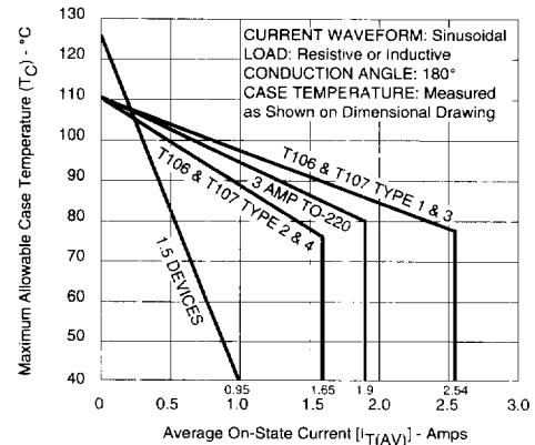
Figure 2B — Maximum Allowable Case Temperature vs Average On-State Current
