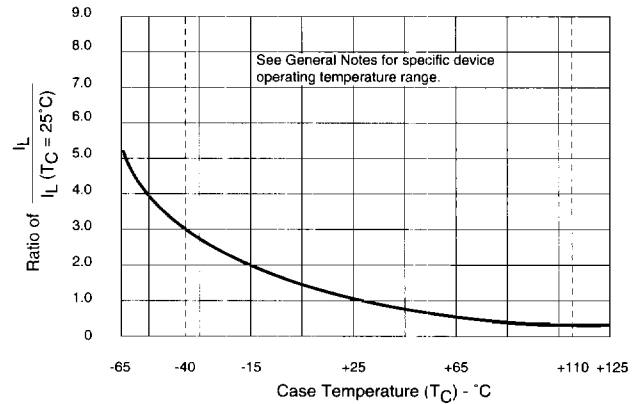
Figure 14 — Normalized DC Latching Current vs Case Temperature
