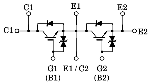
EQUIVALENT CIRCUIT
