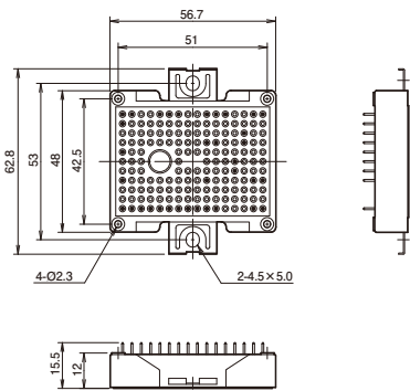
Solder pins
