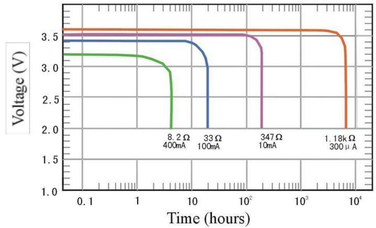
Discharge Characteristics at 23±2°C
