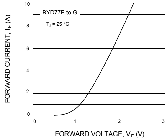
FIG.8 - FORWARD CURRENT AS FUNCTION OF FORWARD VOLTAGE
