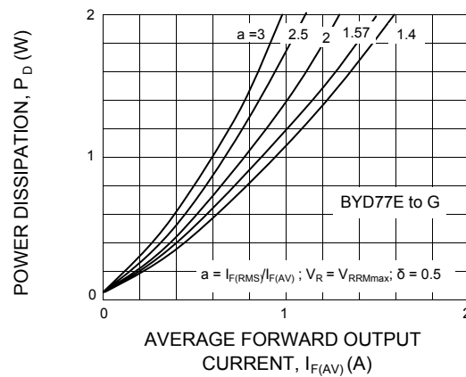
FIG.6 - MAXIMUM STEADY STATE POWER DISSIPATION AS A FUNCTION OF AVERAGE FORWARD CURRENT
