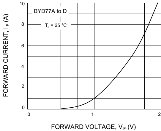
FIG.7 - FORWARD CURRENT AS FUNCTION OF FORWARD VOLTAGE
