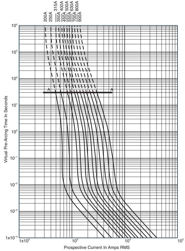
Time-Current Curve
